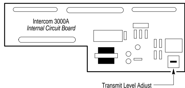
Intercom 3000B Interface Circuit Board Layout
