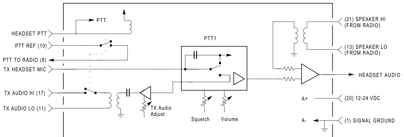
Functional Block Diagram: Intercom 3000B
